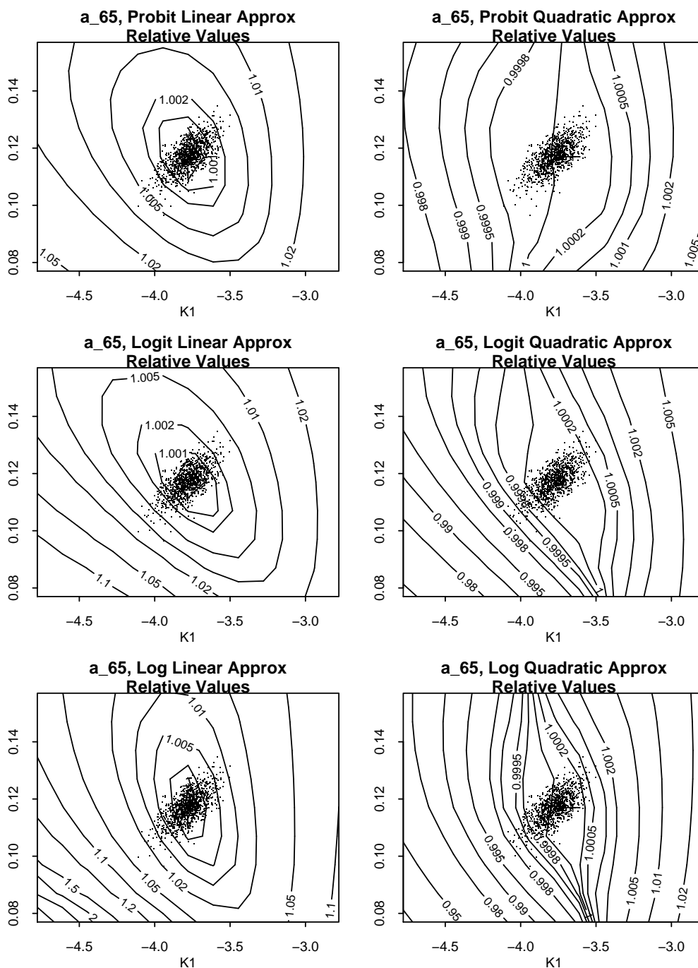
Figure 11: Approximate versus actual values for the annuity function: \hat{a}_{65}(k)/a_{65}(k) . Left-hand plots: Linear approximation. Right-hand plots: Quadratic approximation. Top row: Probit transformation, \Phi^{-1}(x) . Middle row: Logistic transformation, \log(x/(1-x)) . Bottom row: log transformation, \log(x) . The cloud of dots shows 1000 simulated values of the pair (K_1(\tau), K_2(\tau))' for \tau = 20 years after 2008.
